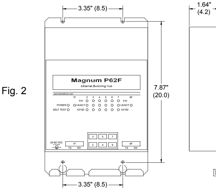
Mounting Hole Dimensions, inches & (cm)
